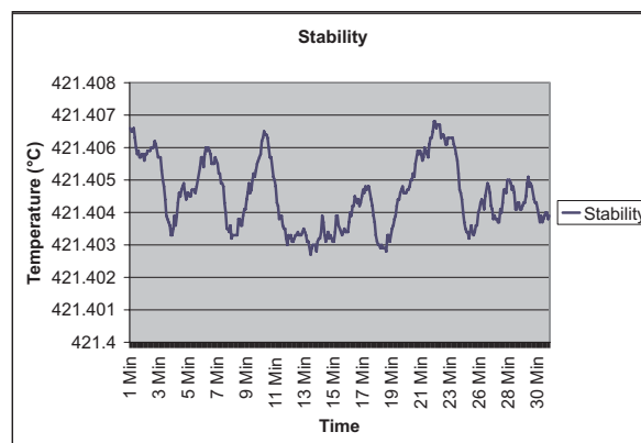
Figure 1. The Metrology Well display can help determine when stability is reached, but a better practice is to rely on display of the reference that offers more resolution.
