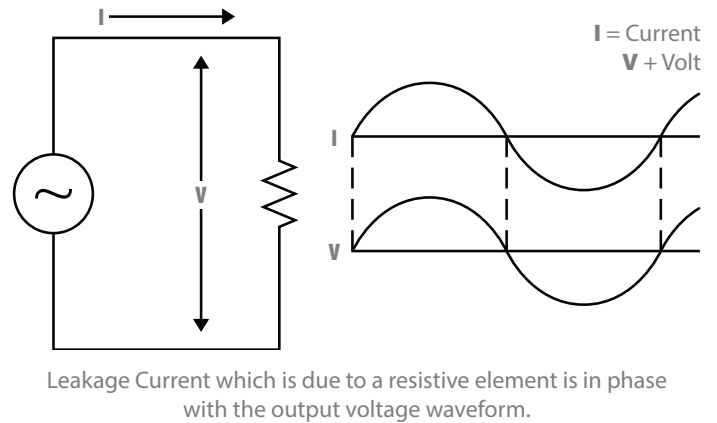
FIGURE 8 CAPACITIVE CURRENT
