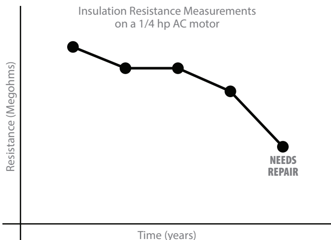
FIGURE 21 DEGRADATION TRACKING
