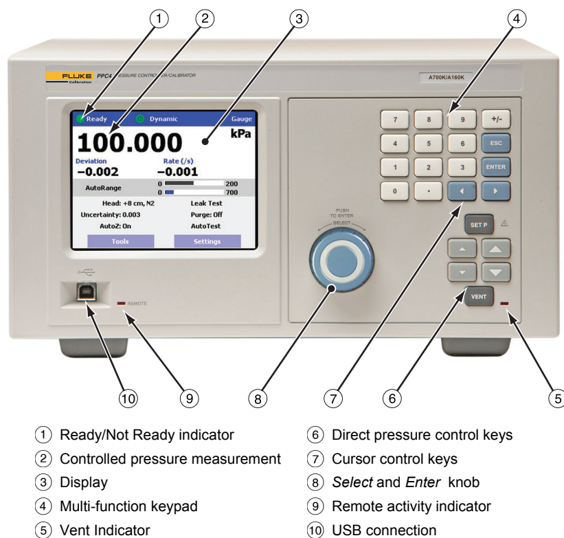
Figure 1. PPC4 advanced interface front panel
