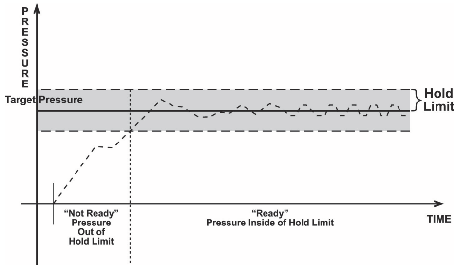
Figure 6. Ready/Not Ready in Dynamic Pressure Control Mode
