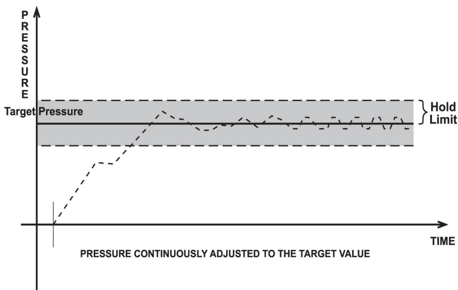
Figure 4. Dynamic Pressure Control Operation
