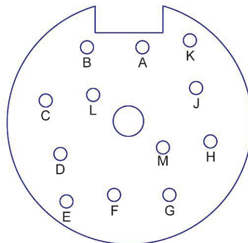
Figure 33. Drivers Connector Schematic
