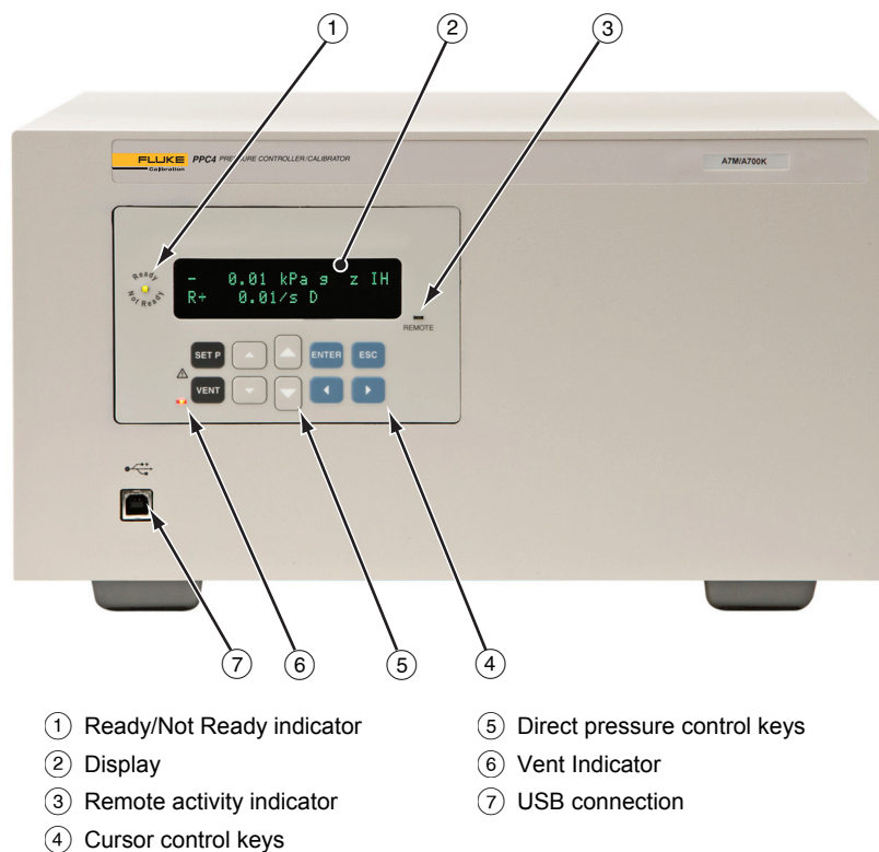
Figure 2. PPC4 basic interface front panel
