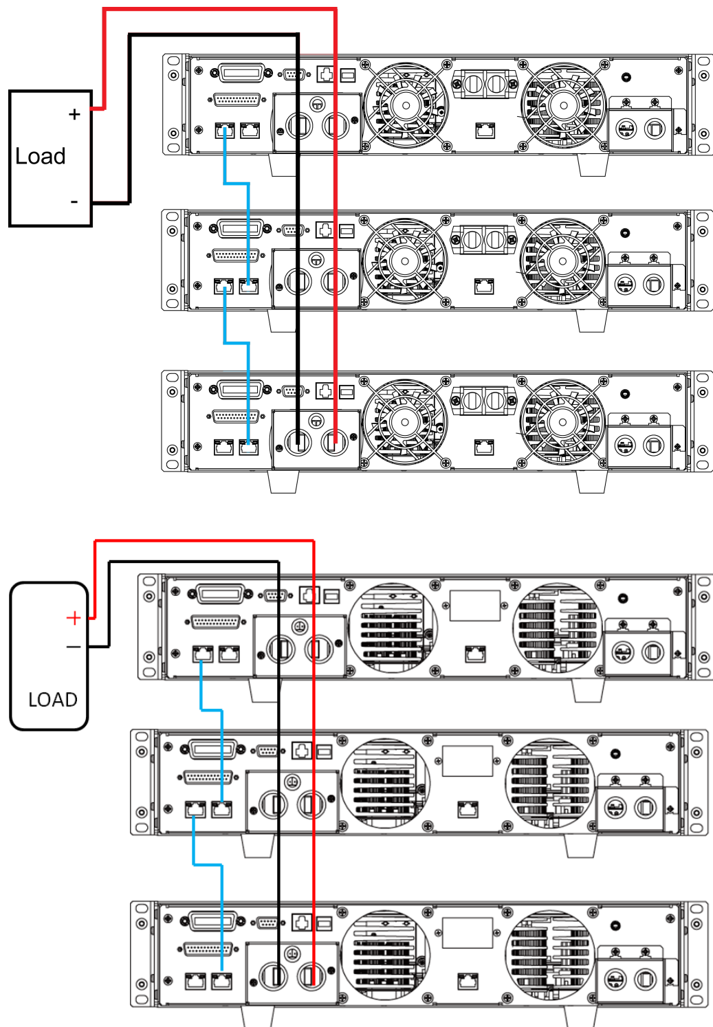
Figure 3–1 Schematic Diagram of 3 Pcs Power Supplies in Parallel
