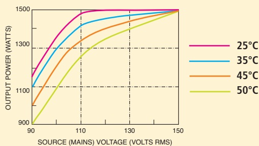
FIGURE 6 HSP 1500W Output Power vs. Source Voltage for Various Ambient Temperatures
