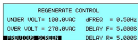
Programming sink (-SNK) mode operation
