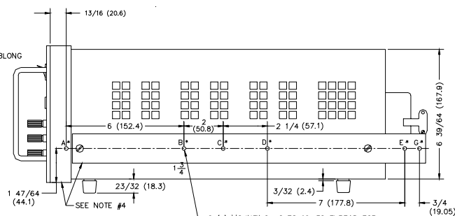
*) MOUNTING HOLES 10-32 THREAD FOR JONATHAN SLIDES SERIES 110 QD (BOTH SIDES, SEE TABLE 1 FOR MOUNTING INSTRUCTIONS
