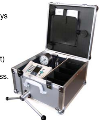
Pressure comparison pump LSP 1000-K
