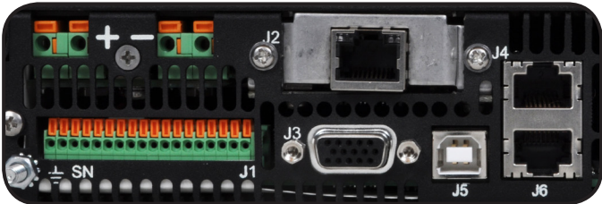
Quick-connect spring-terminal-block
